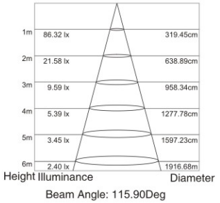
Lux-Distance Curve
