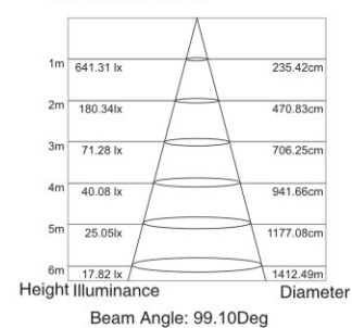
Lux-Distance Curve
