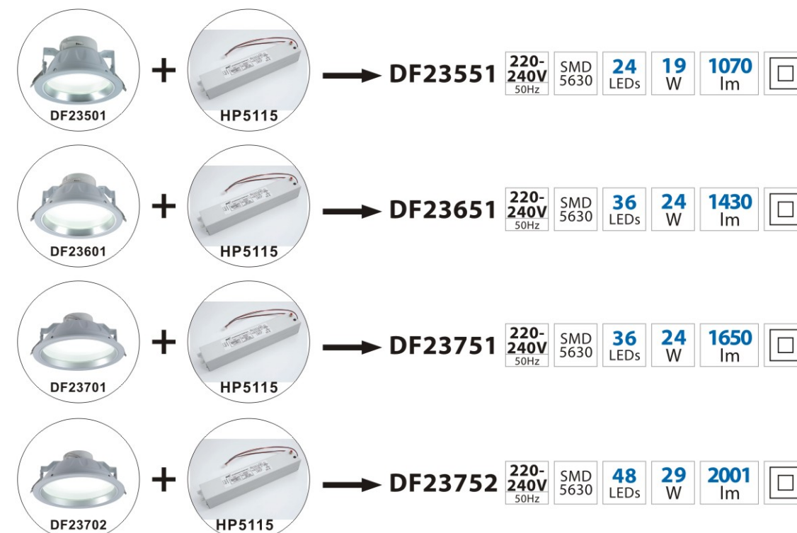
HP5115 Emergency Power Pack
