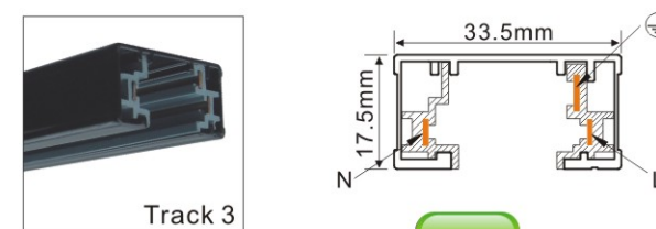
3-Wire Single Circuit Tack
