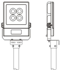
Installation Drawing 2
